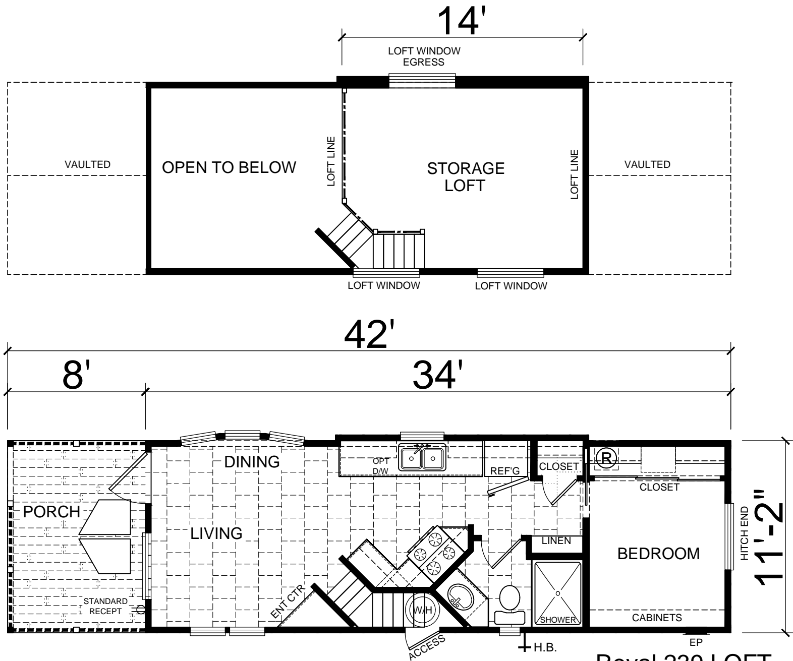
Royal 239 LOFT TOTAL AREA: 398 SQ. FT. REVISED 01/06/2016
